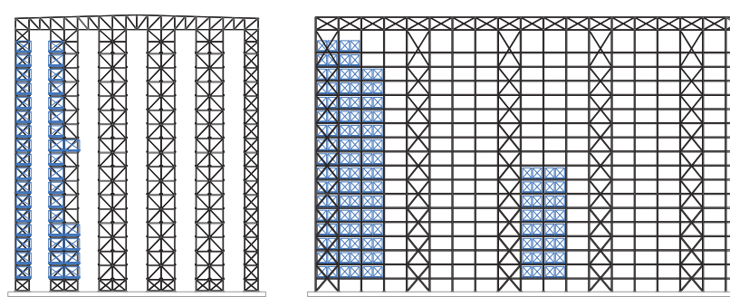
Fig. (2). Transversal and longitudinal sections of the ARSW case-study building. A generic distribution of pallet is also presented.
