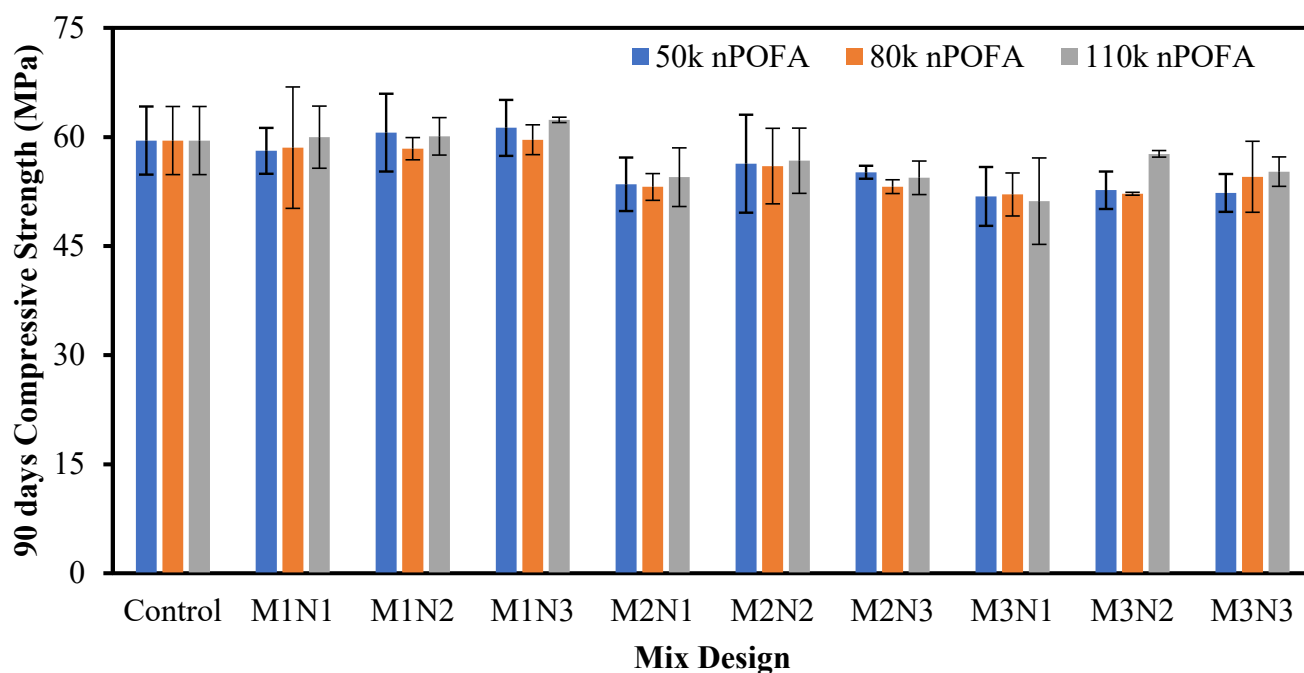
Fig. (8). Compressive strength of all mortars at the curing age of 90 days.
