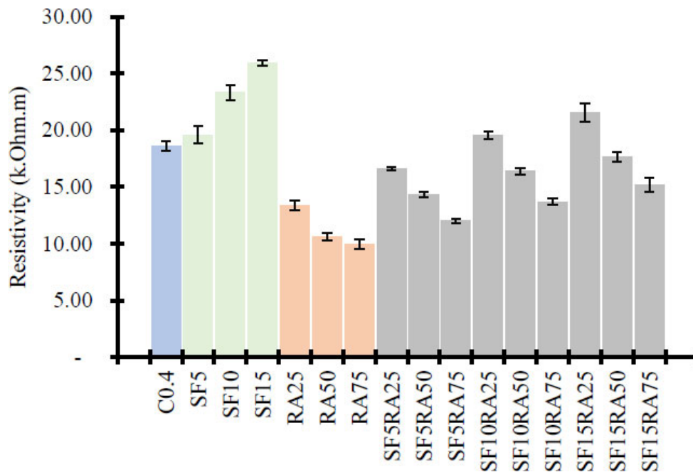
Fig. (7). Electrical resistivity of various mixtures.
