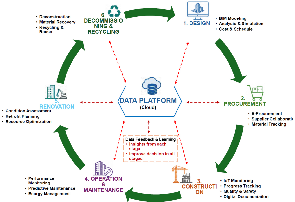
Fig. (1). Landscape of the closed-loop smart construction.
