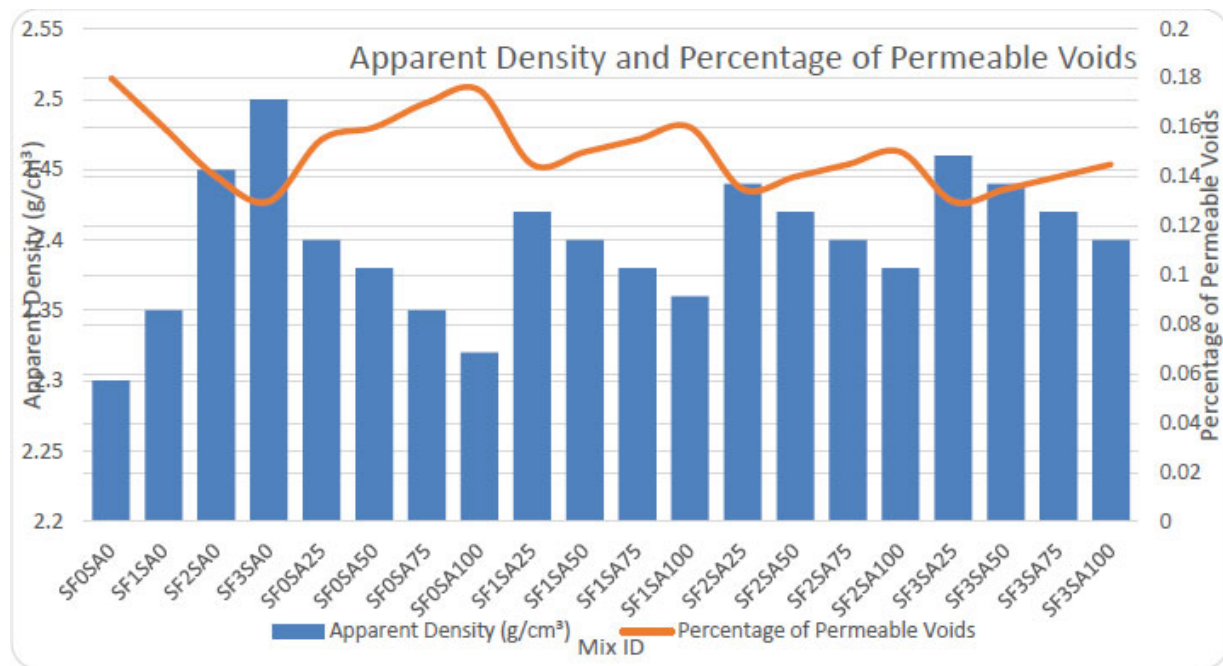
Fig. (10). Comparison of apparent density and percentage of permeable voids in concrete with different percentages of coarse aggregate replacement.
