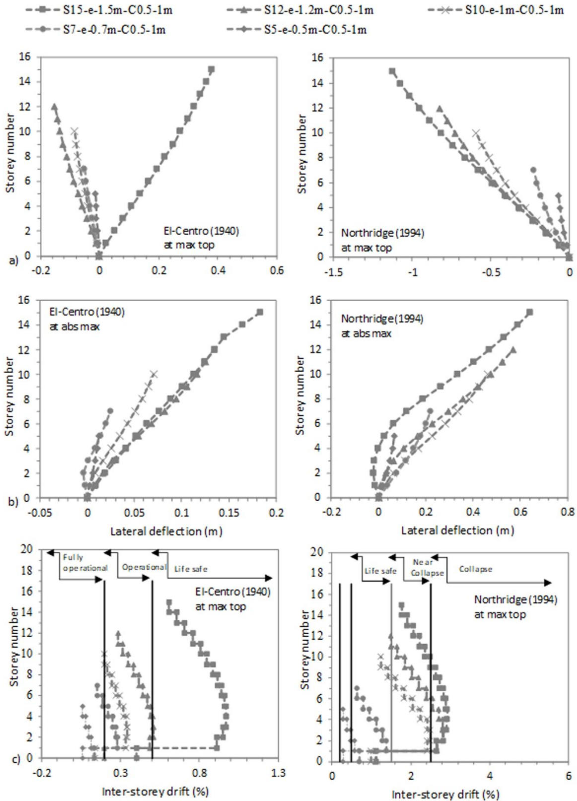
Fig. (7). Variation of lateral deflection a) at max top and b) at abs max and c) Variation of inter-storey drift at max top with storey number for C 0.5 X 1 m flexible structures -effect of structure's number of storeys.
