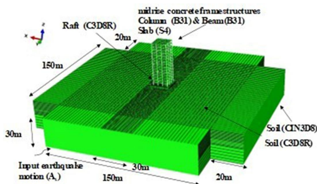
Fig. (1). Geometry and model mesh distribution.
