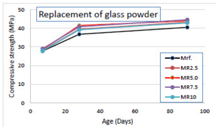
Fig. (4). Development of compressive strength with different weight percentage additions of glass powder.
