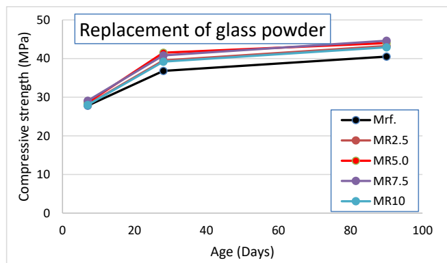
Fig. (2). Development of compressive strength with different weight percentage replacements of glass powder from cement.
