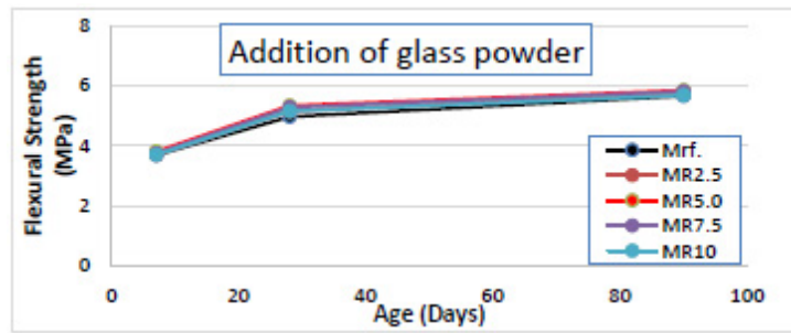
Fig. (6). Development of flexural strength with different weight percentage additions of glass powder.
